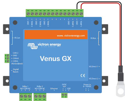
ASS00001000 - Temperature sensor Quattro, MultiPlus and GX Device
